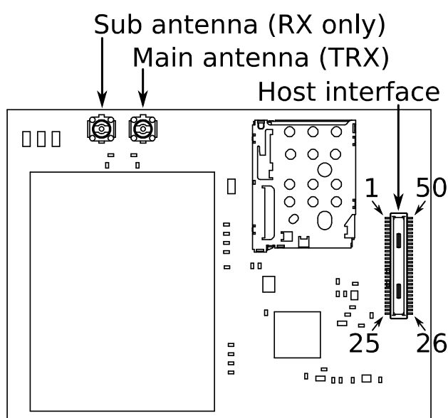
Figure 4 (Top view)
